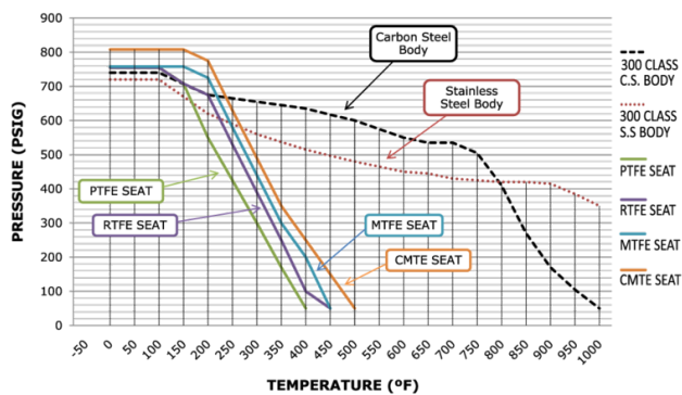
ABZolute - Class 300 Soft Seat - Temp/pressure
